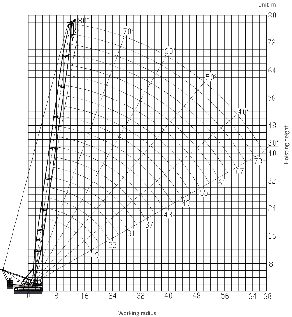
Curves of hoisting height (S)
