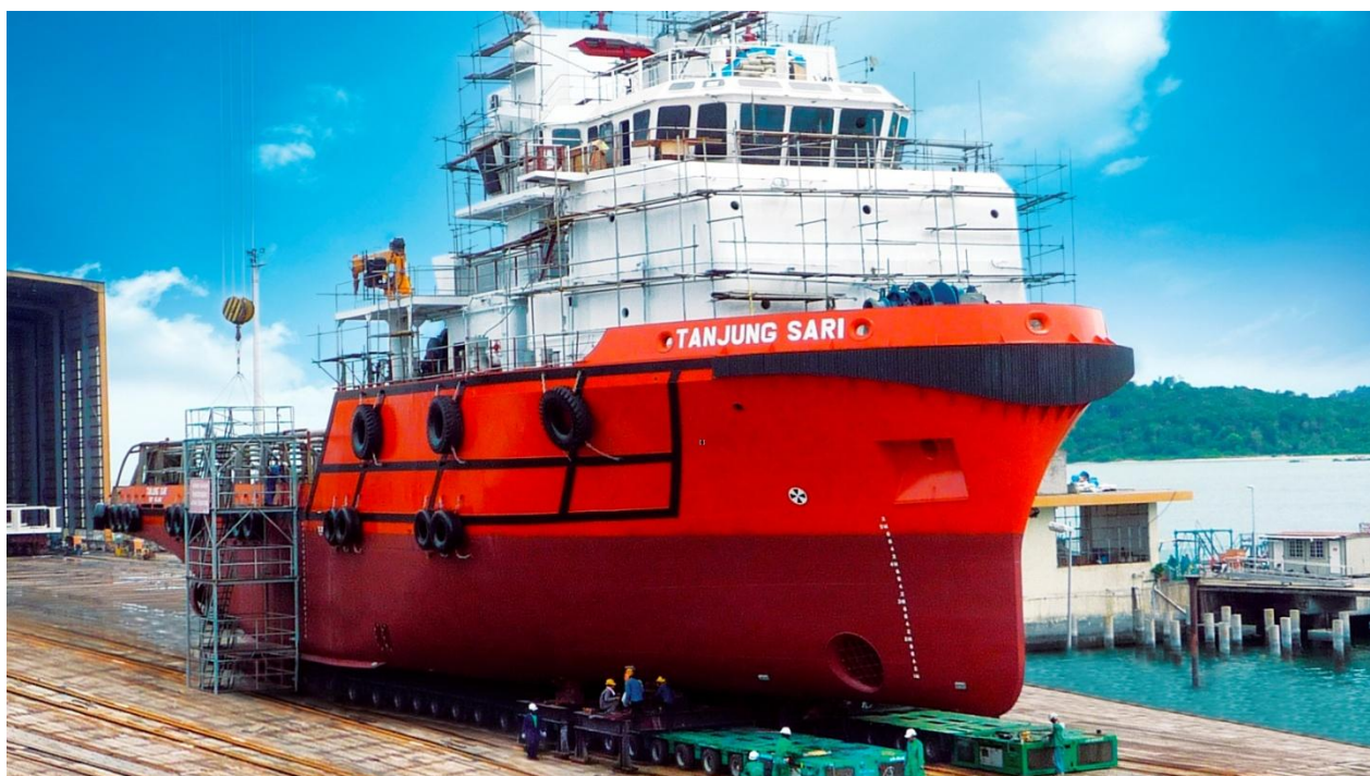
✓ Making a double 90-degree turn maneuver and travelling a distance of 250 metres to the boat-lift-system, the Tanjung Sari Tugboat weighing 1500 tonnes was shifted utilizing 56 axle lines Goldhofer Self-Propelled Modular Hydraulic Controlled Transporter on the 12th July 2009 at Boustead Naval, Lumut Shipyard.
