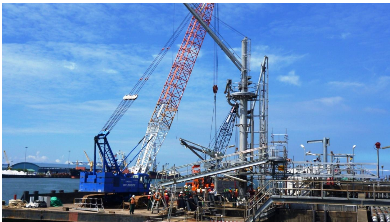
Erection of Sarawak SHELL Berhad's Loading Arm weighing 50 MT utilizing Hitachi KH500 as main crane and Kobelco 7450 as tailing crane.
